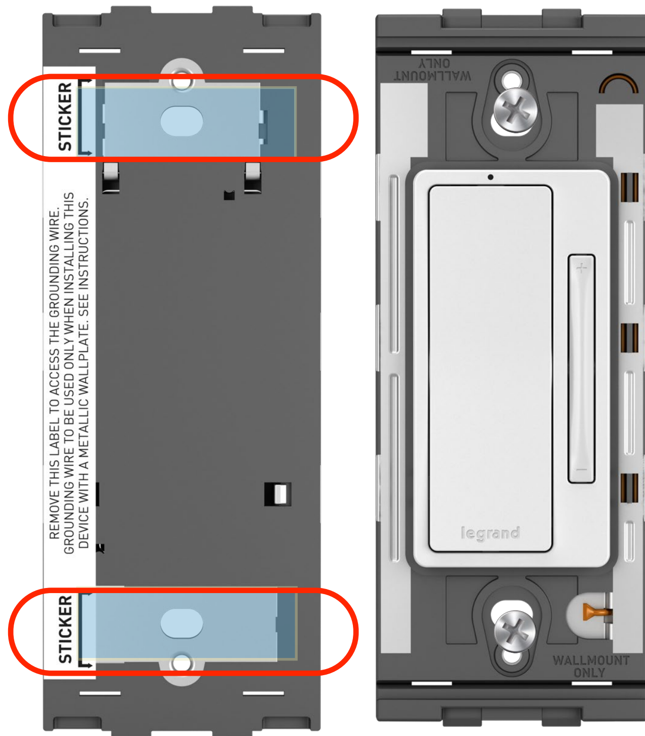
1 Stick it to the wall OR Screw it on the wall
